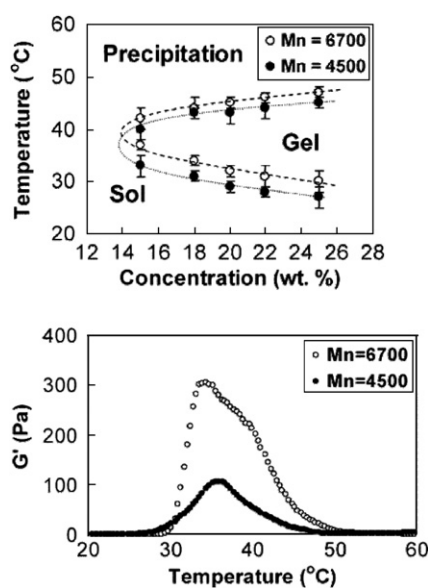
Fig. 7. Influence of total molecular weight of PEG/PLLA multiblock copolymers on the sol–gel transition temperature and storage modulus in aqueous solutions. The modulus was determined for a polymer concentration of 25 wt %. Reproduced from [74] with permission.
