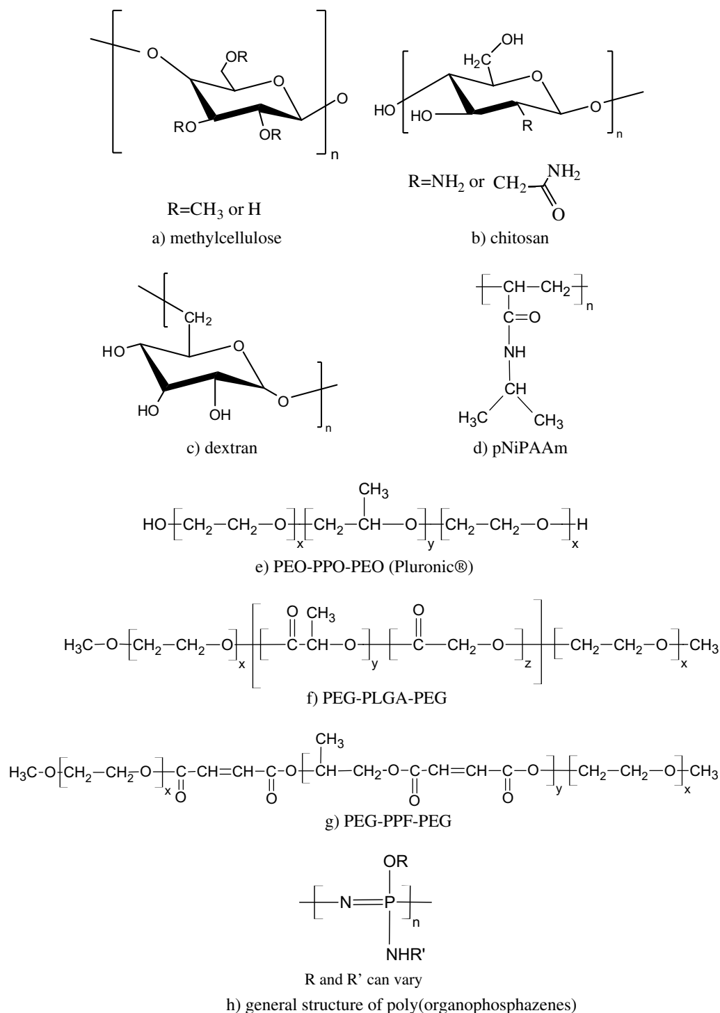
Fig. 1. Chemical formulas of polymers that form or are part of thermoresponsive hydrogels.
