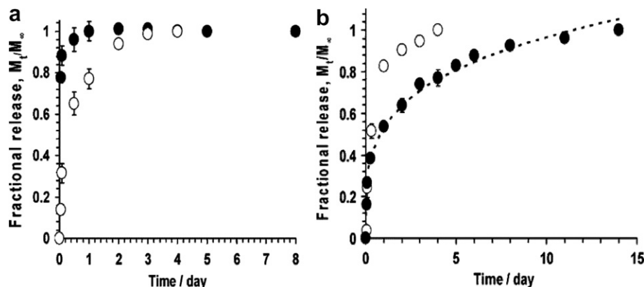
Fig. 3. Fractional release from a hydrogel with 5:4 NiPAAm:Dex-lactate-HEMA weight ratios in PBS of methylene blue (a) and BSA (b) at 25 (○) and 37 (●) °C. Reproduced from [31] with permission.
